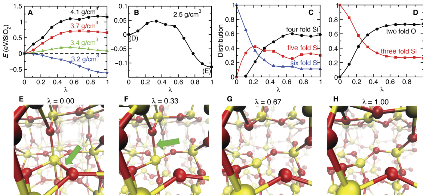
Fig. 4. Amorphization pathways. (A) Energy profile from stishovite crystal (reaction coordinate \lambda = 0 ) to high-density amorphous phase ( \lambda = 1 ) obtained by NEB calculation. The energy for configuration 0 is set to zero. (B) Energy profile for a subsequent amorphous-to-amorphous transformation corresponding to configurations (d) to (e) in Fig. 2A. (C and D) Distributions of the coordination number of Si (C) and O (D) atoms along the reaction pathway, which are calculated using a cutoff distance r_{\text{Si-O}} = 2.2 \text{ \AA} . (E to H) Snapshots of atomic configurations at \lambda = 0 (E), 0.33 (F), 0.67 (G), and 1 (H) along the stishovite-to-amorphous transformation at \rho = 3.4 \text{ g/cm}^3 , corresponding to a transition from (a) to (b) that is shown in Fig. 2A.
